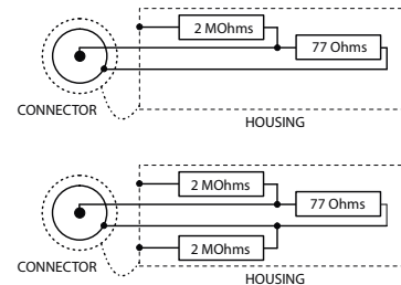
77 Ω TERMINATOR WITH ESD PROTECTION
